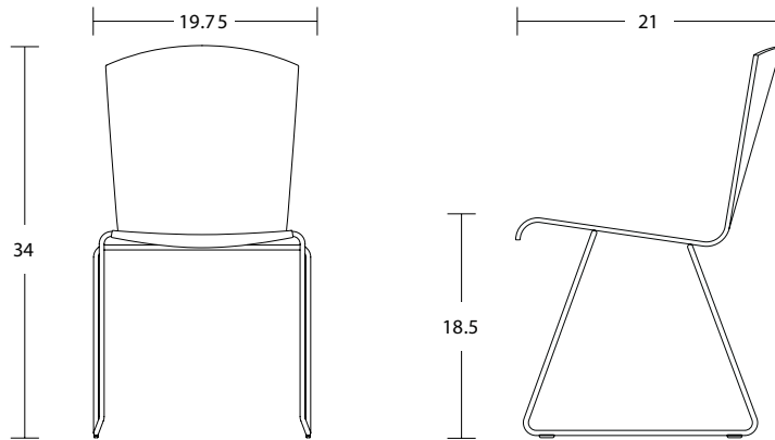
Sled Base, Arc Shell / MQS-A
